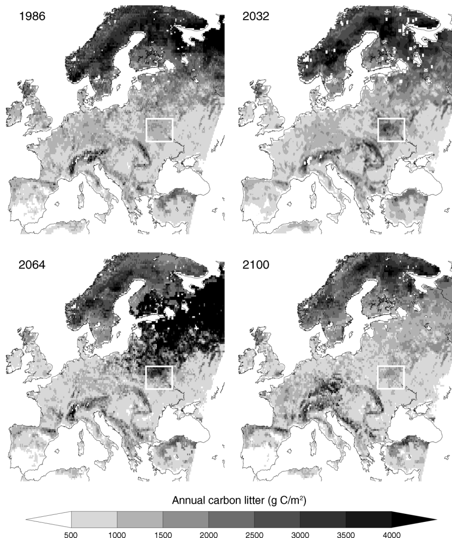
FIG. 11. Litter carbon stock over Europe 1986–2100 based on the future prediction of the LPJmL-SPITFIRE model. White rectangle denotes the contaminated forests in Ukraine and Belarus.
